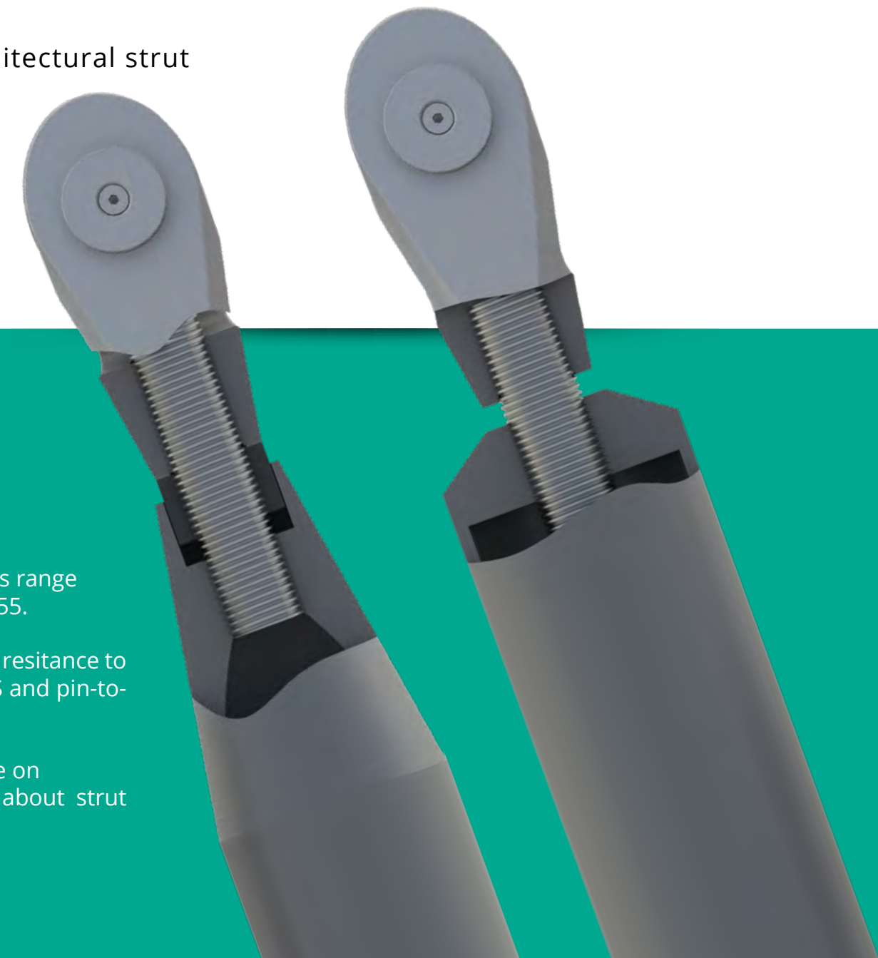
Non-Architectural strut
